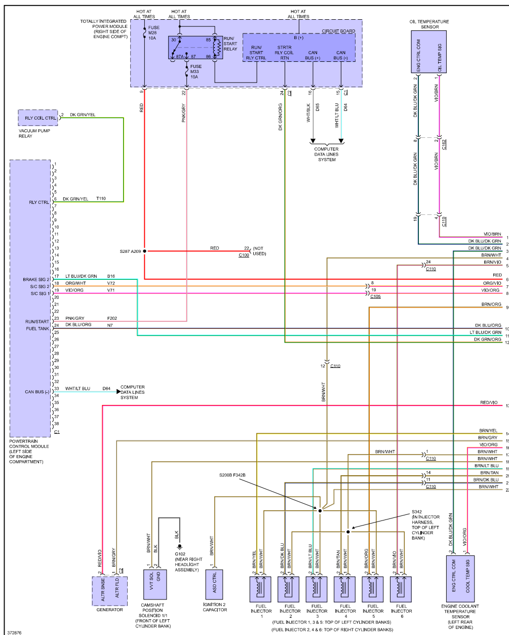
Fig 1: 3.6L, Engine Performance Circuit (1 of 5)
