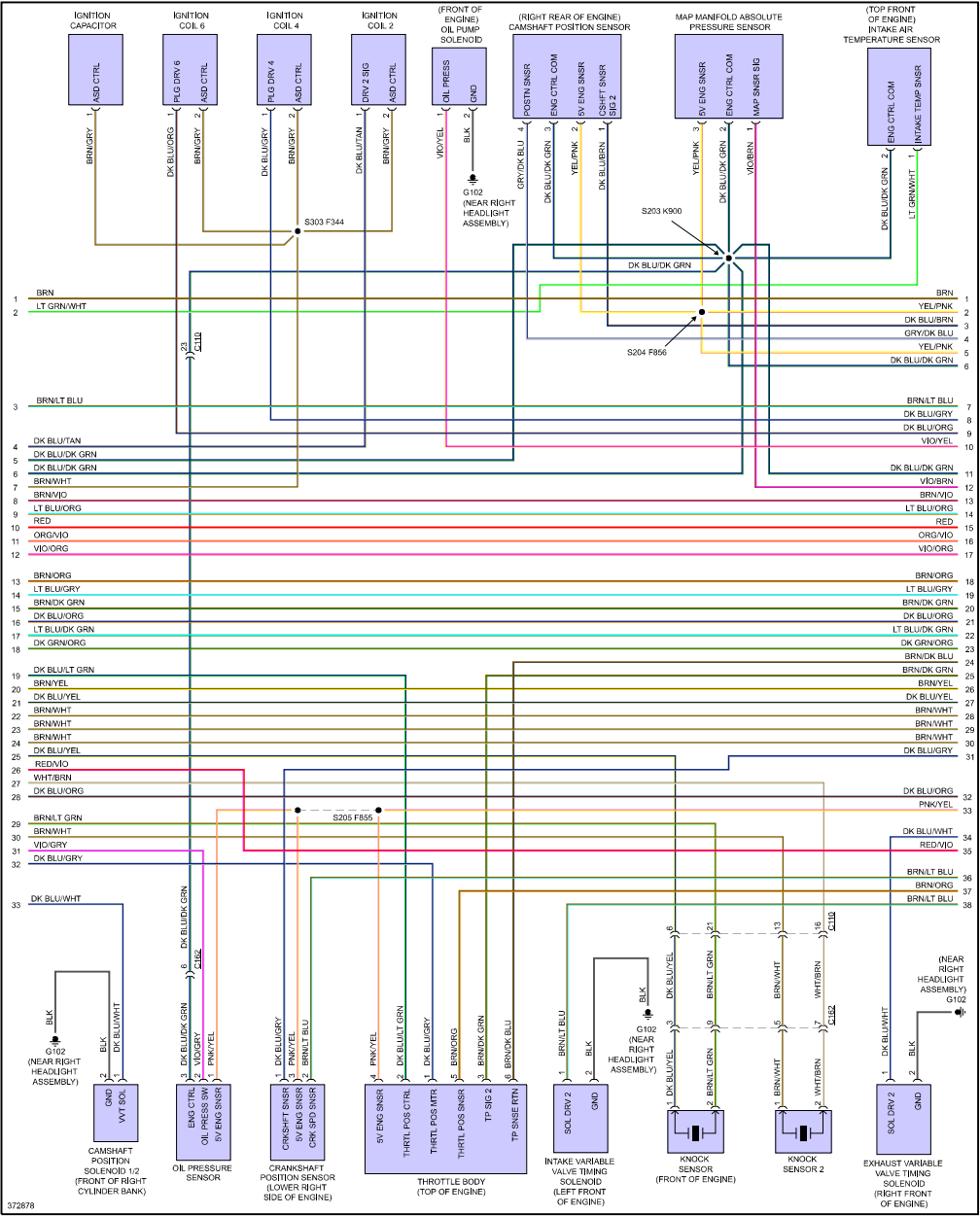
Fig 3: 3.6L, Engine Performance Circuit (3 of 5)
