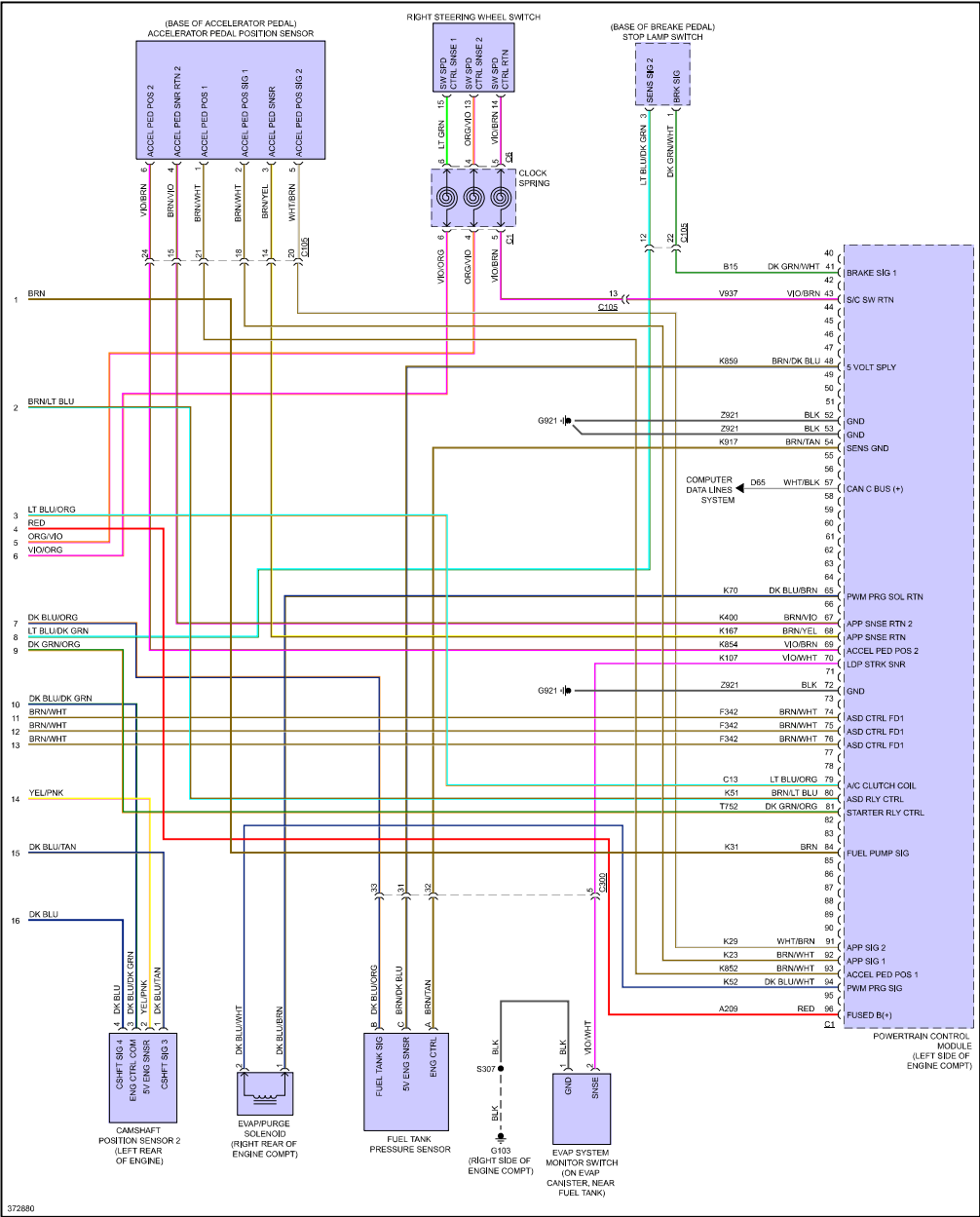
Fig 5: 3.6L, Engine Performance Circuit (5 of 5)
