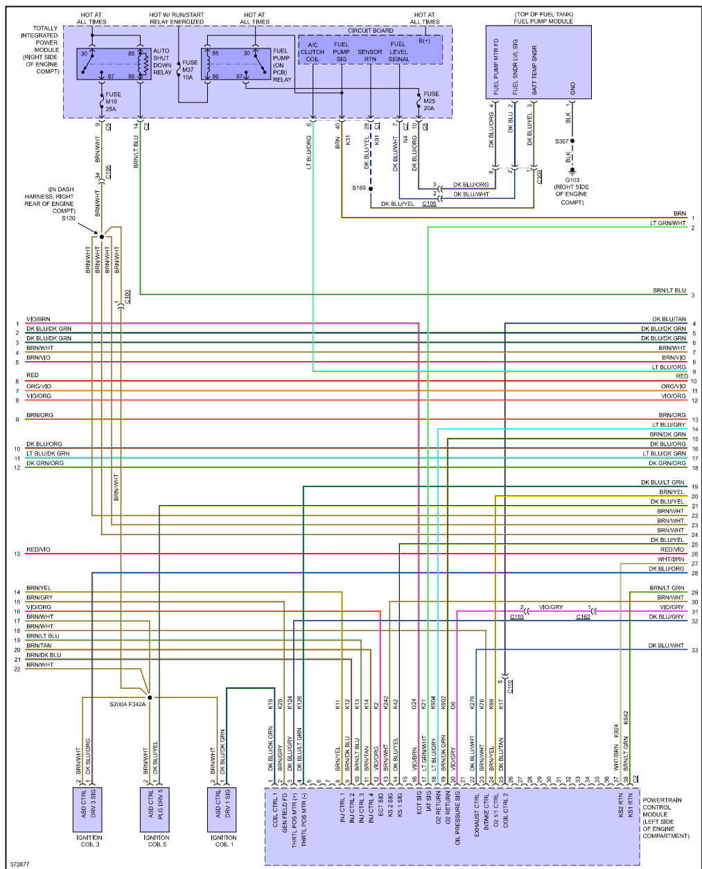
Fig 2: 3.6L, Engine Performance Circuit (2 of 5)
